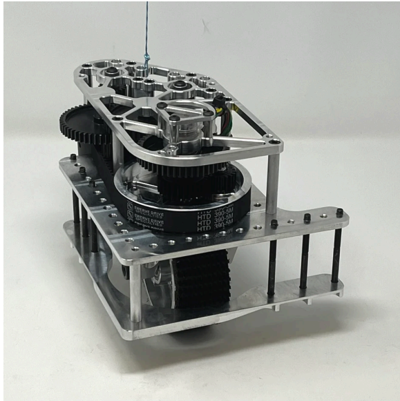
MK4n Swerve Module and FRC Climb 2025:
